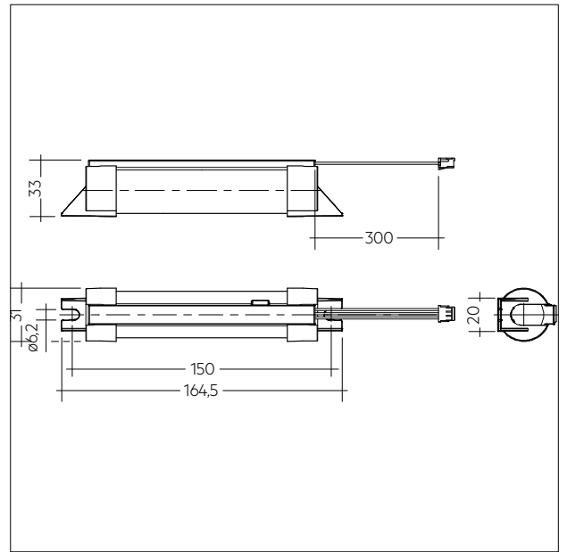
TA_EM_M_Accu_LiFePO4_3_6Ah_2A.wmf
