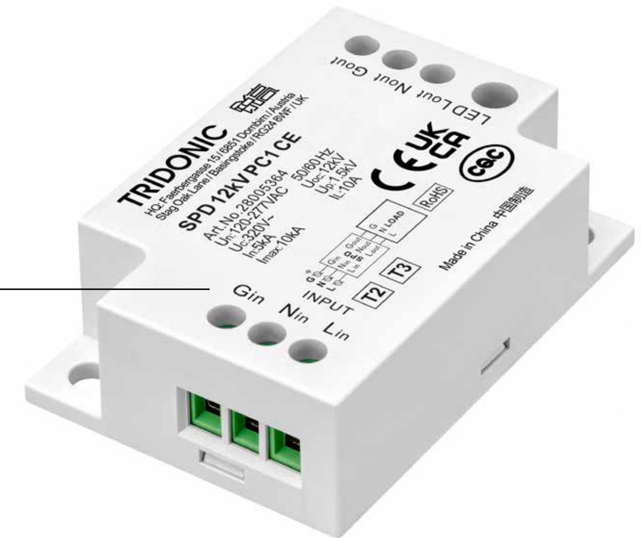
Surge protection device class I
