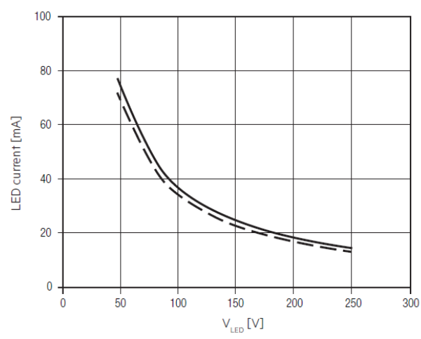
M converterLED PRO 204 NiCd/NiMH 250V
