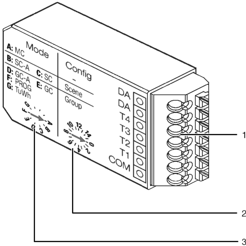
Figure 1: DALI XC input device
