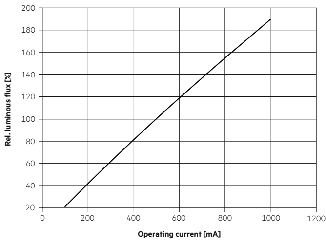
SLE 17mm 5000lm ADV8
