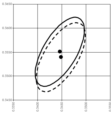
— MacAdam Ellipse: 3SDCM (1,050 mA) - - MacAdam Ellipse: 3SDCM (350 mA)
