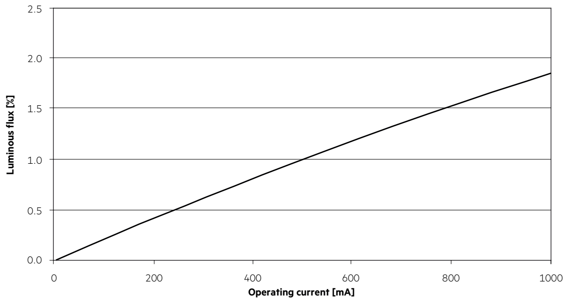
DLE G4 65mm 3000lm 8x0 advanced
